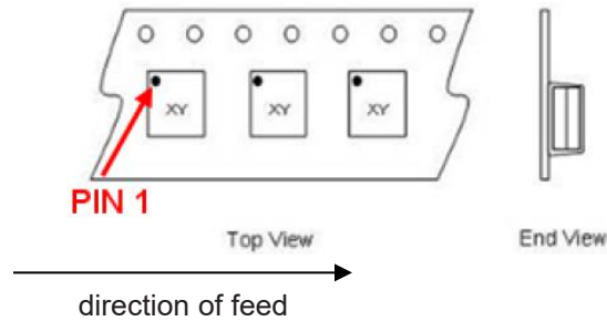
Fig 2. Product orientation in carrier tape
